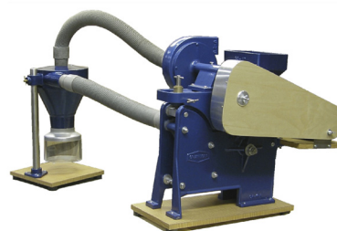
GRAINMAN #64 Rice Sheller USDA Approved
